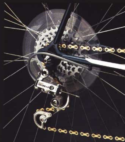
Hi-spec alloy gear system with braze on down tube shifter
