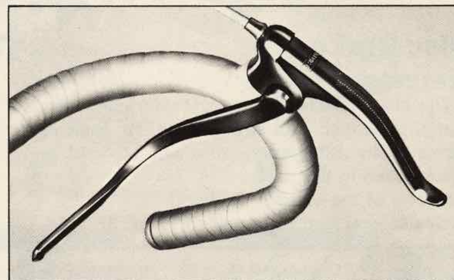
Dual Extension Lever (22.2 \phi ) Model No.: M-210 Dual Extension Lever (23.8 \phi ) Model No.: M-220
