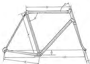
Frame geometry.
