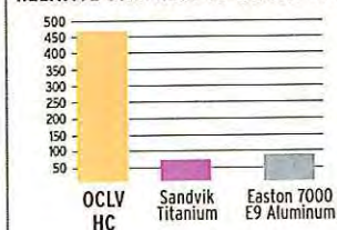
RELATIVE STIFFNESS-TO-WEIGHT RATIO
