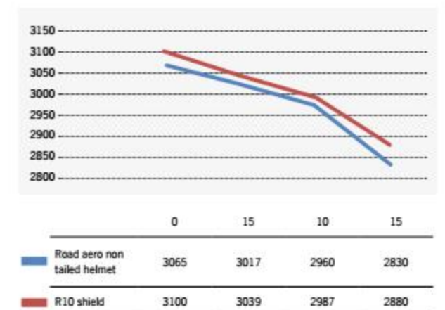
Comparison with aerodynamic road cycling helmets: The R10 is 1% less efficient but 20% more vented. Graphic: R10 vs aerodynamic road cycling helmets.
